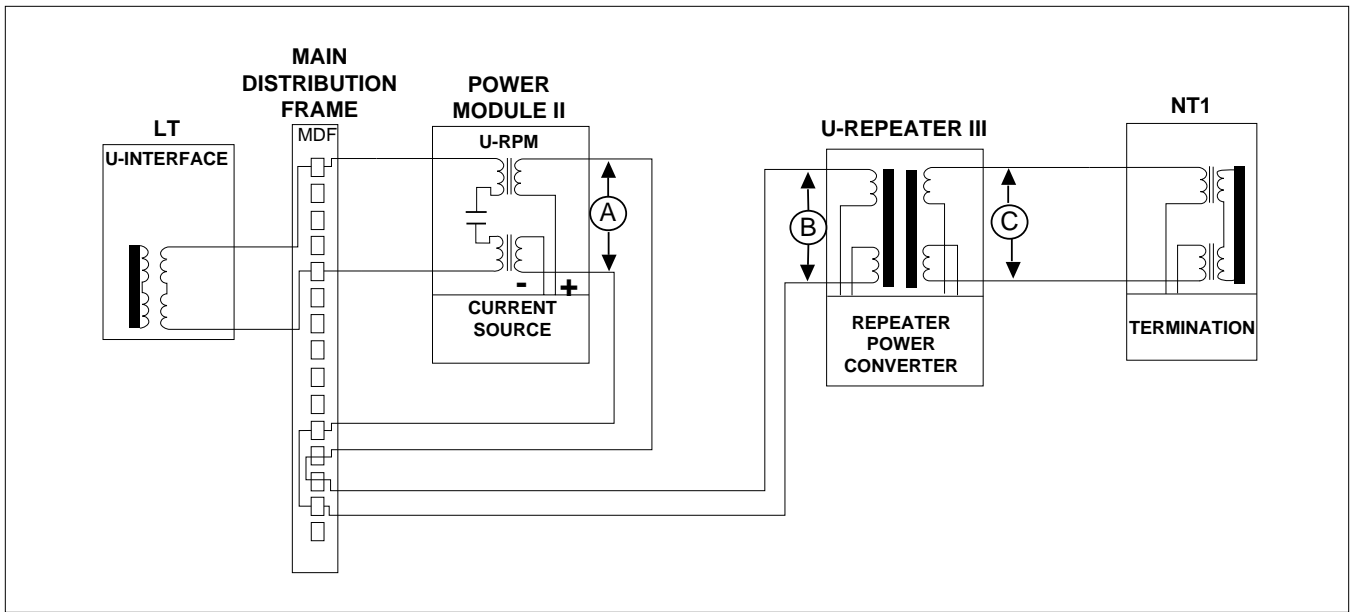
Figure 5. Typical U-Repeater III Circuit Voltage Test Points
