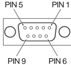
Figure D-2. Modem Interface
