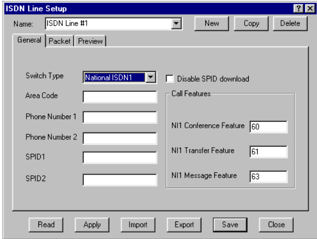
Figure 3-3. ISDN Profile Setup Window
