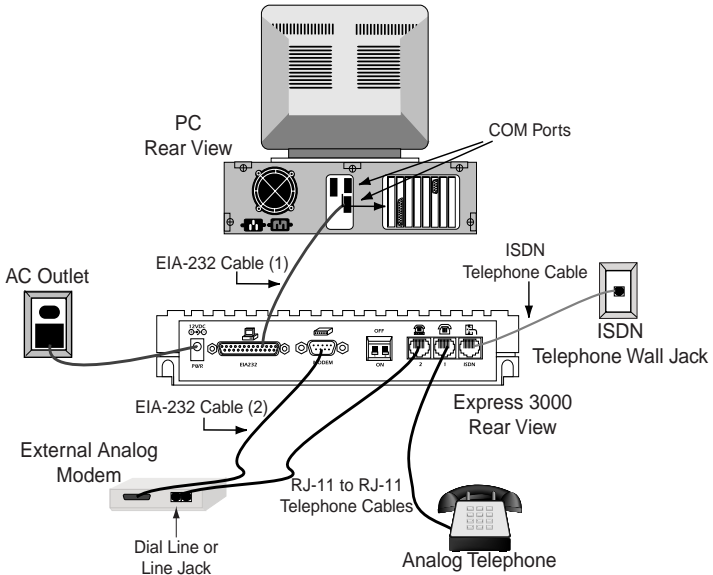
Figure 7-1. External Analog Modem Application
