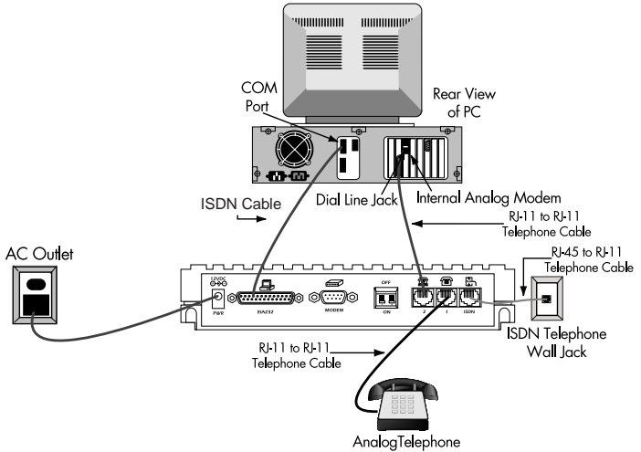
Figure 7-2. Internal Analog Modem Connections
