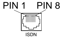
Figure D-4. RJ-45 ISDN Line Interface
