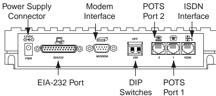
Figure 2-2. Express 3000 Rear Panel
